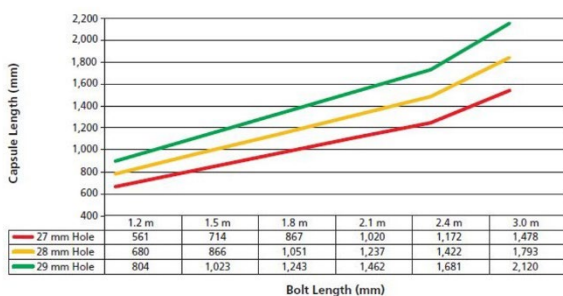
25 mm nominal diameter capsule with 22 mm core diameter bolt Theoretical encapsulation + 10%
