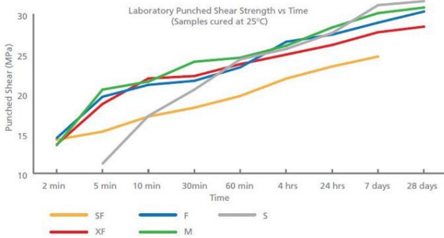
Figure 3 - Laboratory Punched Shear Strength vs Time
